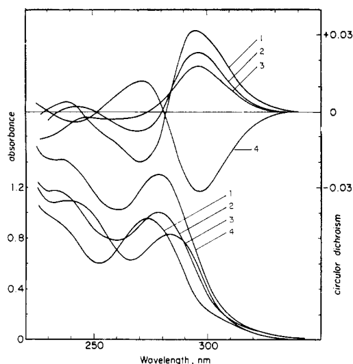
FIGURE 1: Circular dichroism (measured on a Cary 60 recording spectropolarimeter equipped with CD attachment 6002 at 23°, corrected against buffer-blank and expressed in \text{deg cm}^2 \mu\text{mol}^{-1} ; upper set of spectra) and absorbance (lower set of spectra) for [3-(2-amino-2-carboxyethyl)-3-(8-xanthinyl)indolenines]: (1) isomer IIIa, pH 1.0; (2) isomer IIIa (pH 7.4); (3) isomer IIIa, pH 11.0 (solutions 1–3 are of the same concentration); (4) isomer IIIb, pH 7.4.
