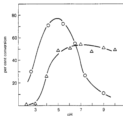
FIGURE 2: Dependence of the formation of xanthine adducts IIIa plus IIIb (O) and "tryptophan oxidation products," ( \Delta ) on pH; 3 mg of 3-acetoxyxanthine dissolved in 0.05 ml of \text{Me}_2\text{SO} and 30,000 cpm of [\beta\text{-}^{14}\text{C}]\text{-L-tryptophan} ( 122 \times 10^6 \text{ cpm}/\mu\text{mol} ) were reacted for 30 min at 37° in 0.3 ml of buffer (0.1 M each of \text{H}_3\text{PO}_4 , HOAc, and glycine, pH adjusted with 10 N NaOH to pH values from 2.3 to 10.0). The yield of IIIa and IIIb was determined from their radioactivity after paper chromatography ( \text{BuOH-HOAc-H}_2\text{O} , 5:1:4, asc.). The yield of "oxidation products" was determined in the first 7.0 ml of \text{H}_2\text{O} eluate of small 1.0-ml columns of Dowex 50 [\text{H}^+] over which the reaction mixture was chromatographed. A control experiment involved ^{14}\text{C} tryptophan added to a reaction mixture of 3-acetoxyxanthine in buffer pH 7.0 after preincubation for 30 min, and was negative for both types of products.
